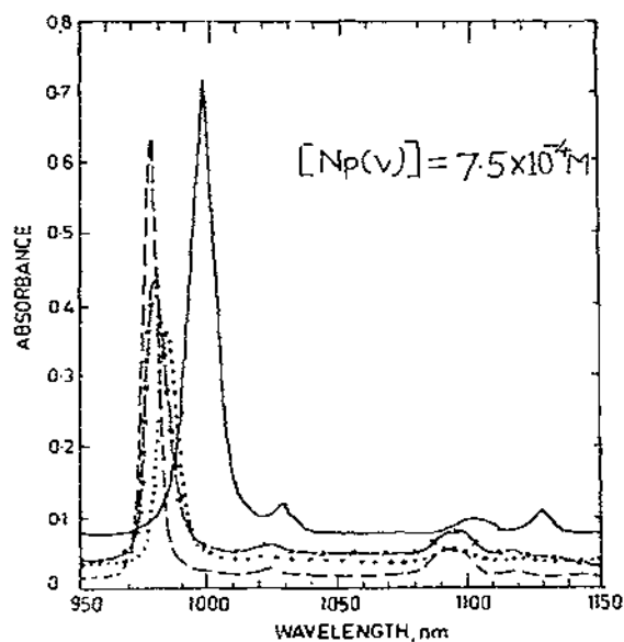
Fig. 2. Absorption spectra of Np(V) obtained using 2.0 cm cells in 6.6 M \text{NaClO}_4 (----), 0.05 M \text{NaF} (-·-·-), 3.0 M \text{Na}_2\text{SO}_4 (.....) and using 1.0 cm cells in 8 M \text{NaSCN} (—) [49a].
