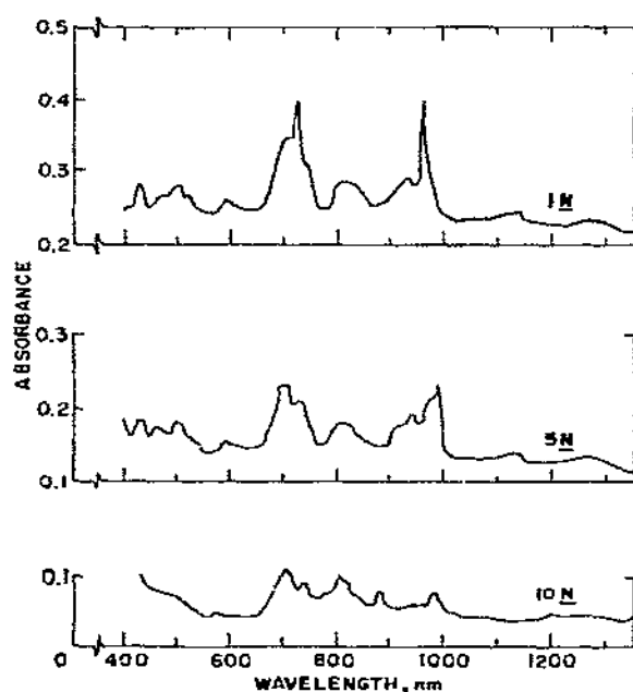
Fig. 4. Absorption spectra of Np(IV) in 1.5 and 10 M nitric acid ( [Np(IV)] = 2.0 \times 10^{-3} M 1.0 cm cells) [97].
