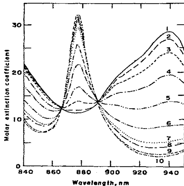
Fig. 5. Absorption spectra of Np(IV) in nitric acid in region of 877 nm peak: (1) 5.0 M HNO_3 , (2) 6.0 M HNO_3 , (3) 7.0 M HNO_3 , (4) 8.0 M HNO_3 , (5) 9.0 M HNO_3 , (6) 10.0 M HNO_3 , (7) 11.0 M HNO_3 , (8) 12.0 M HNO_3 , (9) 13.0 M HNO_3 , (10) 14.0, 15.0 and 15.5 M HNO_3 . Reprinted with permission from J. Phys. Chem., 64 (1960) 1375. Copyright by the American Chemical Society.
