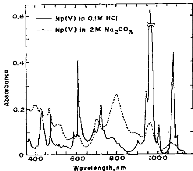
Fig. 12. Absorption spectra of Np(V) ( [\text{Np(V)}] = 2.2 \times 10^{-1} \text{ M} , 1.0 cm cells) [152]. Reprinted with permission from Akademai Kaido.
